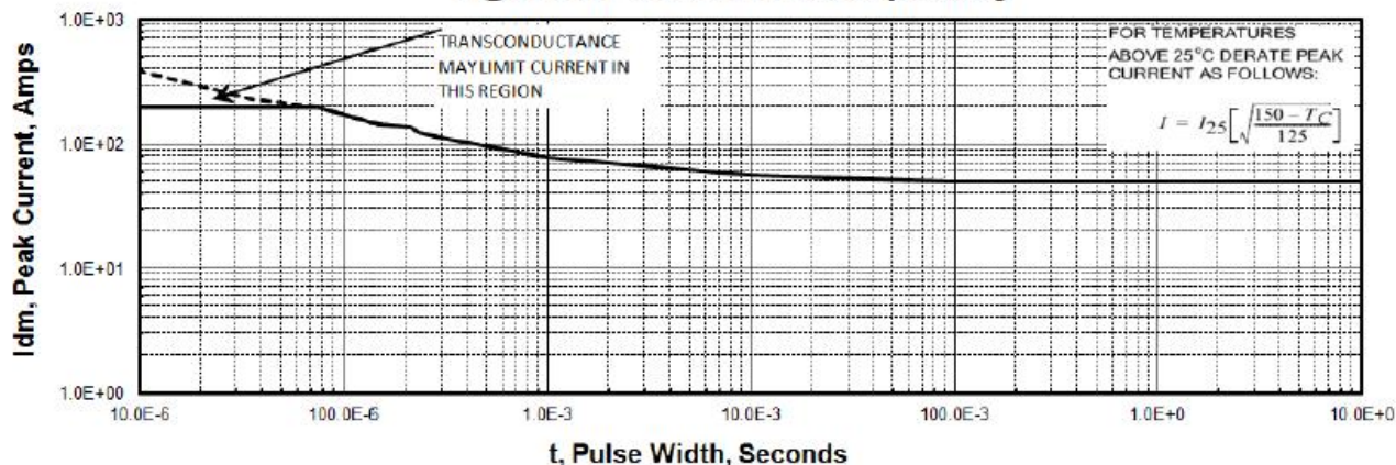
Figure 7. Transfer Characteristics
