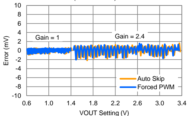
V_{OUT} Setting Accuracy ( I_{OUT} = 10mA )
