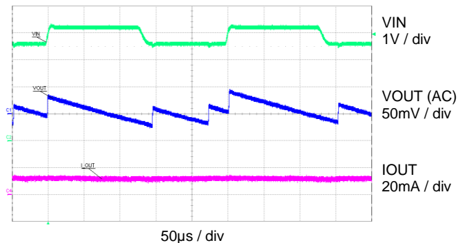
Line Transient Response (V OUT = 1.136V, Mode = Auto)
