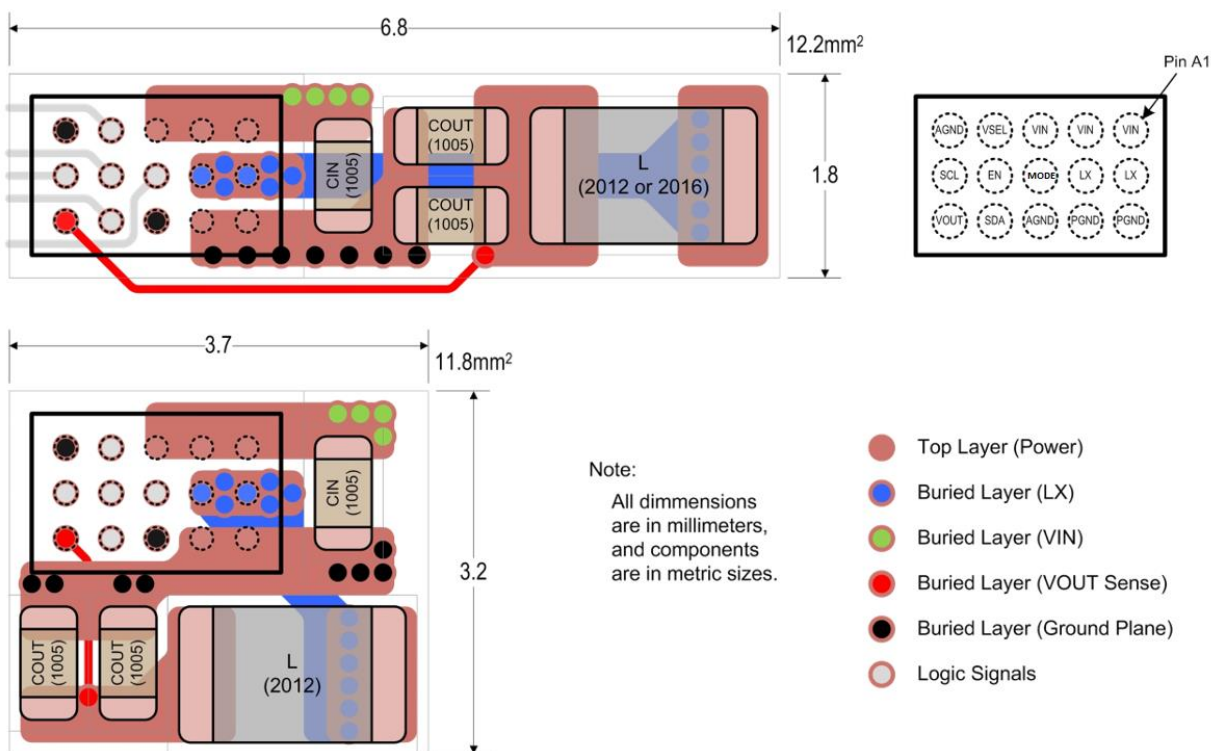
Figure 6. Two Recommended PCB Layouts
