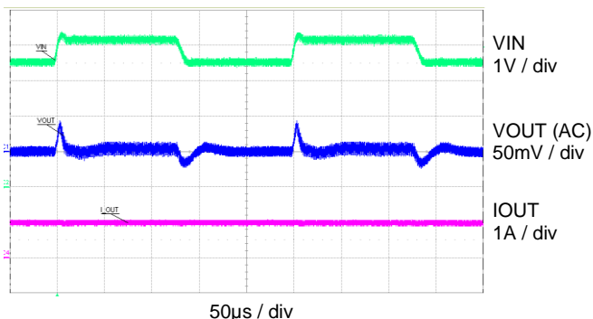
Line Transient Response (V OUT = 1.136V, Mode = FPWM)
