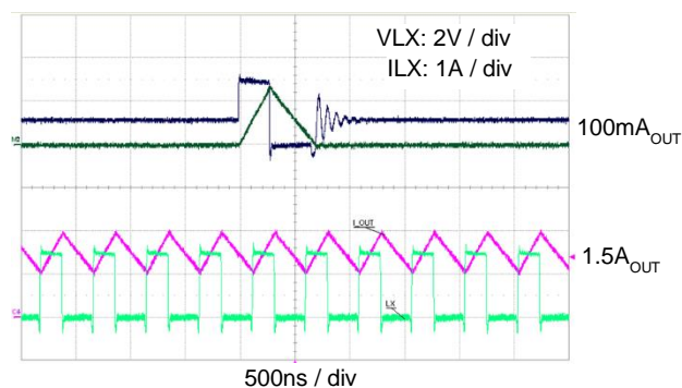
V_{LX} and I_{LX} Switching Waveforms ( V_{OUT} = 1.136V , Mode = Auto)
