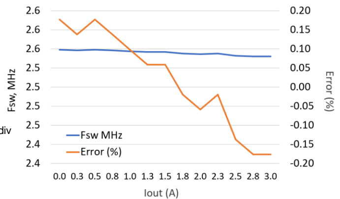
Switching Frequency Accuracy vs Iout ( V_{OUT} = 1.136V )
