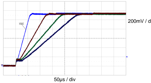
Buck Enable Soft-Start Rates ( V_{OUT} = 1.136V )
