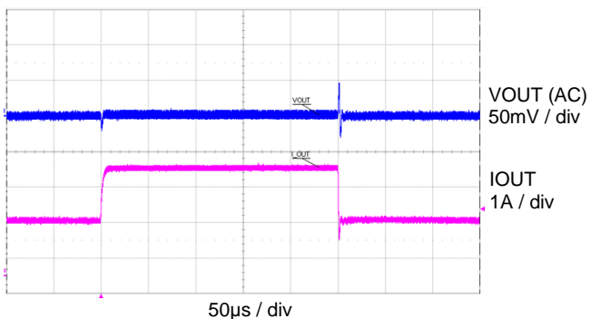
Load Transient Response (V OUT = 1.136V, Load = 1.5A-3A, Mode = Auto)
