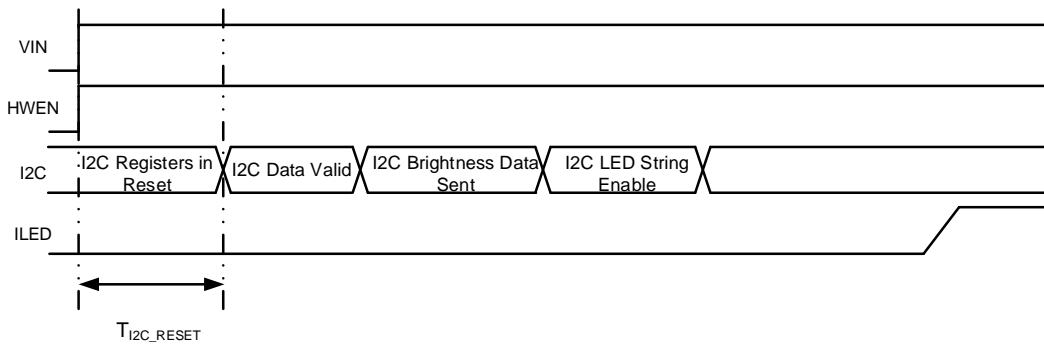
Figure 2. Enable of KTZ8864 via I 2 C
