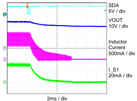
Turn Off by I 2 C
