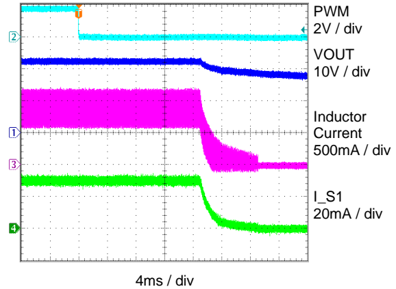
Turn Off by PWM
