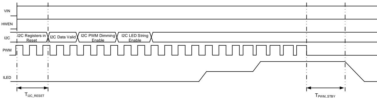
Figure 3. Enable of KTZ8864 via PWM
