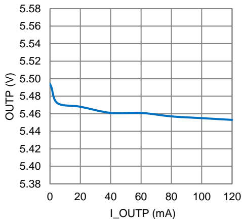
OUTP Load Regulation
