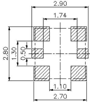
Recomend PCB Layout General Tolerance: \pm 0.05
