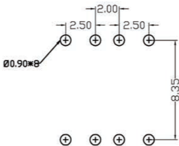
RECOMMENDED P.C.B PATTBRN LAY OUT
