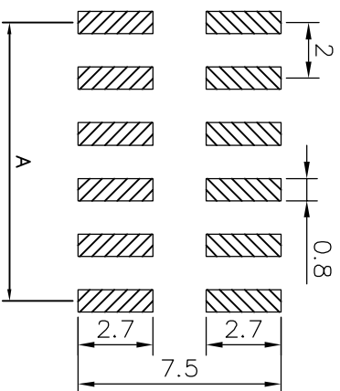
RECOMMEND P. C. B LAYOUT PCB TOLERANCE: ±0.05 (TOP VIEW)
