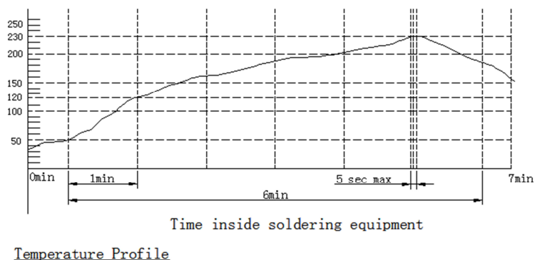
Temperature Profile
