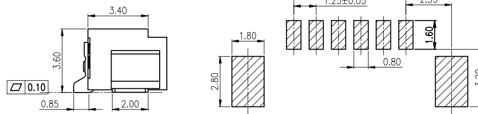
PCB LAYOUT
