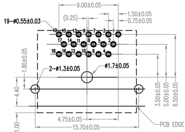
RECOMMENDED PCB LAYOUT SCALE 3:1
