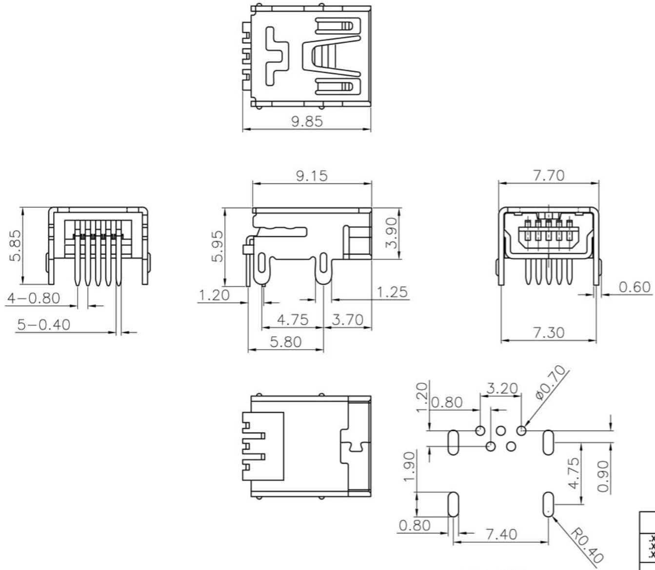
PCB LAYOUT
