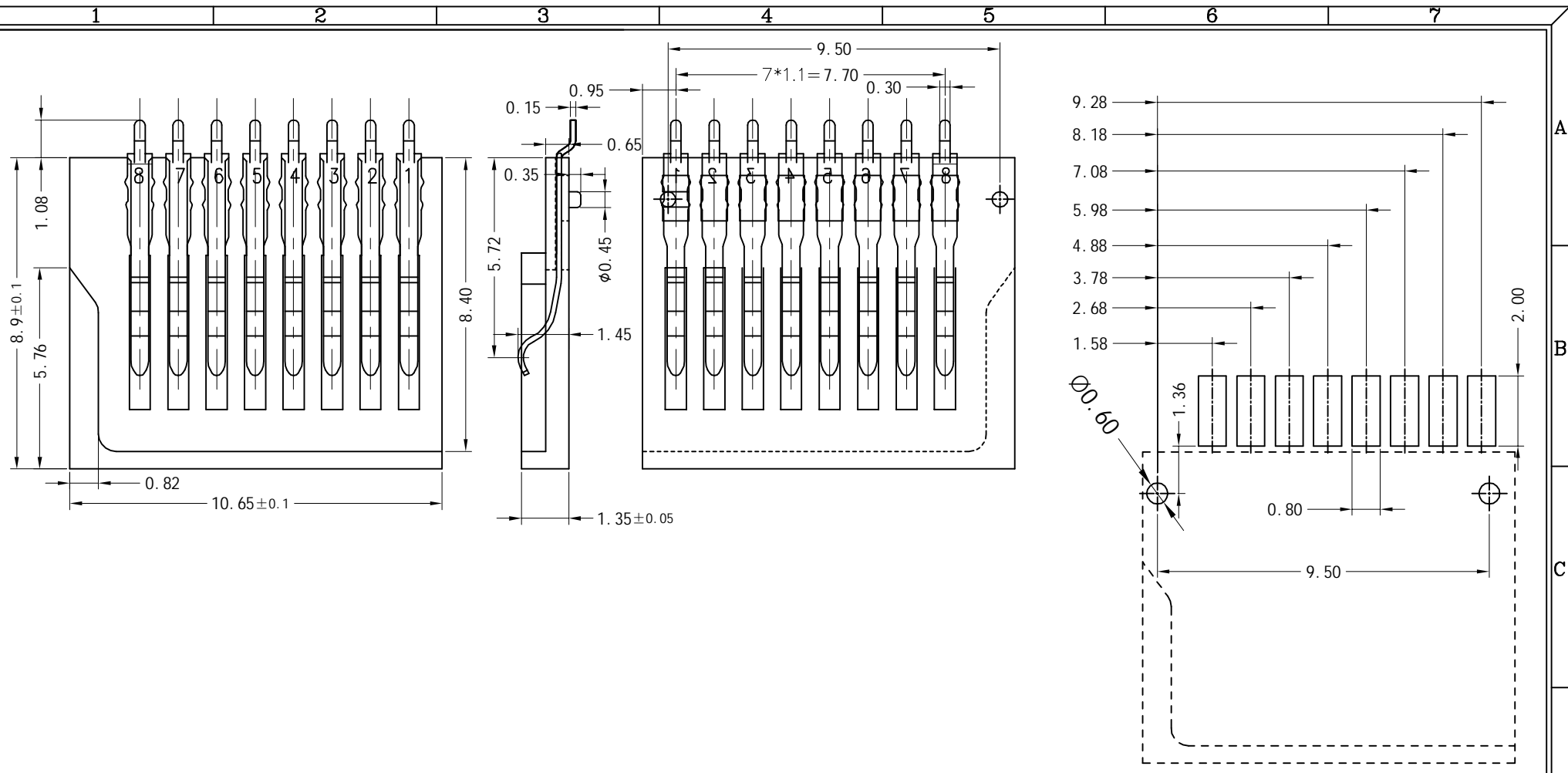
P. C. B LAYOUT
