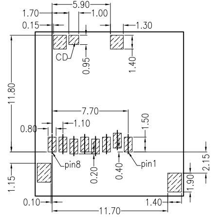
RECOMMENDED P.C.B HOLE LAYOUT COMPONENT SIDE VIEW(TOLERANCE: +/-0.05)
