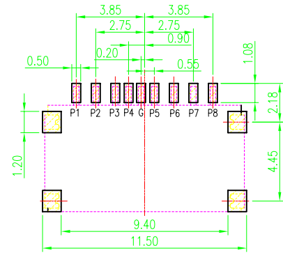
RECOMMEN P.C.BOARD LAYOUT GENERAL TOLERANCE ±0.05
