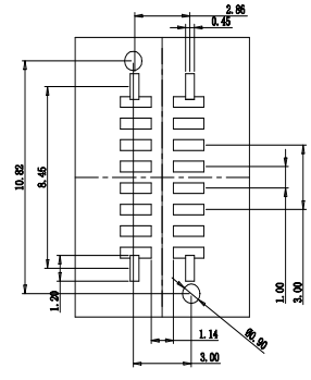
RECOMMENDED P.C.B. LAYOUT (T:1.00mm) TOLERANCE UNSPECIFIED \pm 0.05mm
