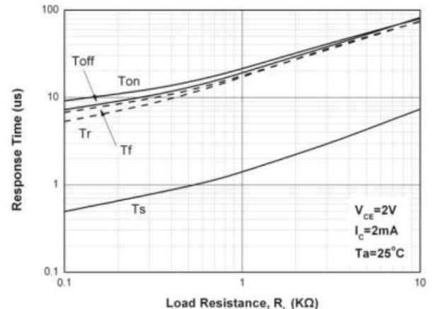
Fig.6 Switching Time vs Load Resistance
