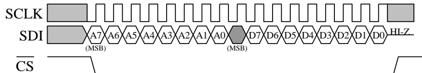
Figure 9: Timing Diagram for 8-Bit Register Read Operation
