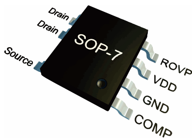
SOP-7
