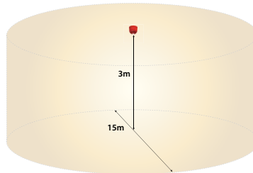
EN54-23 Coverage: C-3-15
