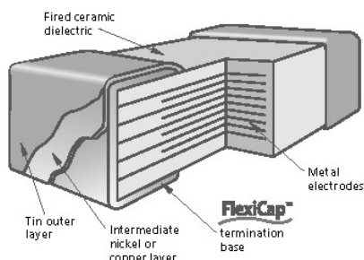
FlexiCap™ MLCC cross section
