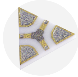
Left: Example of a Wilkinson Power Divider PDW Right: Example of a Resistive Power Divider PDR (note: shows mounting configuration on bottom side of the part)
