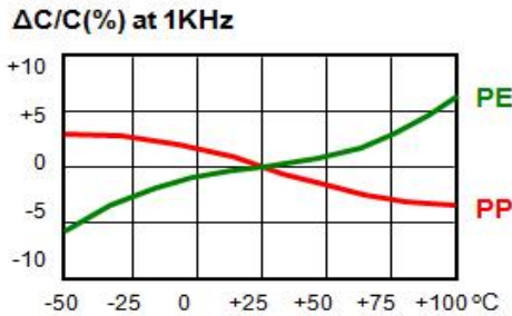
Temperature Characteristics
