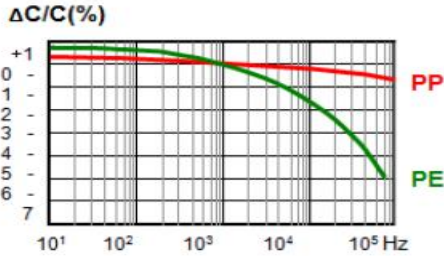
Frequency Characteristics
