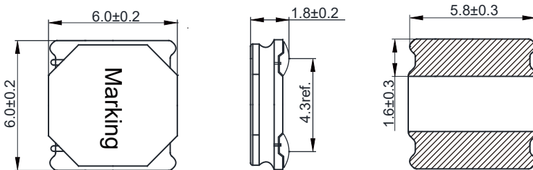
Dimensions: [mm]
