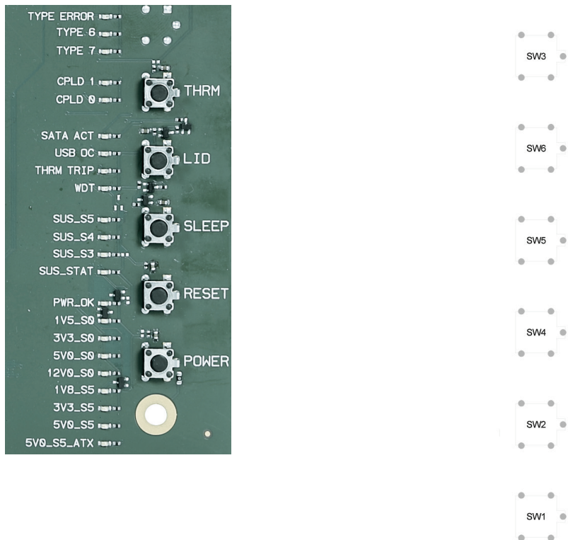
Figure 20: Button Switches
