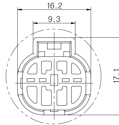
DETAIL Z(2/1)
