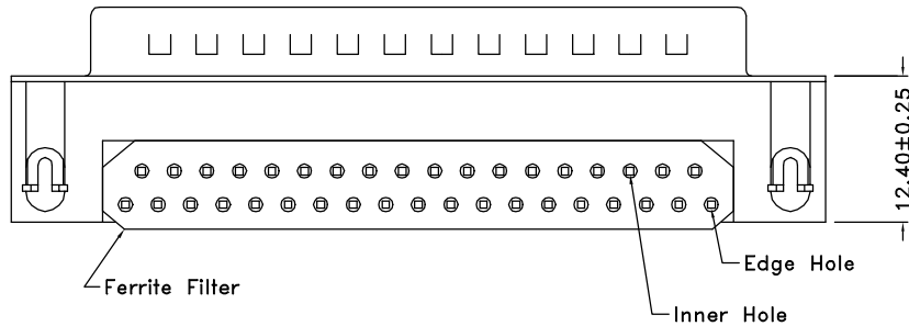
Recommended PCB Layout (Bottom View)
