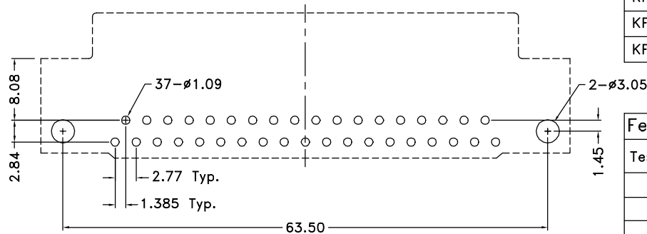
Recommended PCB Layout (Bottom View)
