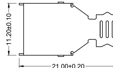
Back Shell
