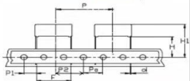
Fig 4 Pitch: 22.5/27.5 Po=12.7
