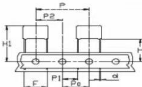
Fig 3 Pitch: 10/12.5/15 P=12.7
