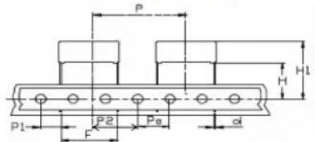
Fig 4 Pitch: 22.5/27.5 P=12.7
