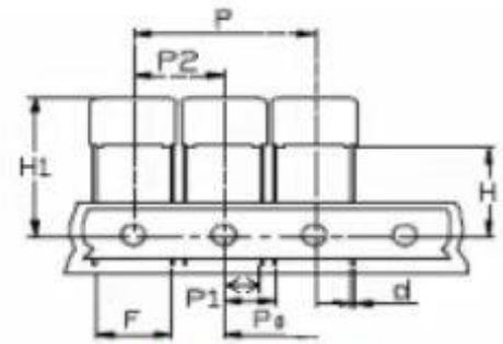
Fig 2 Pitch: 7.5 P=12.7 Pitch: 10.0 P=15.0
