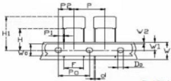
Fig 1 Pitch: 5.0 P=12.7 Pitch: 7.5 P=15.0
