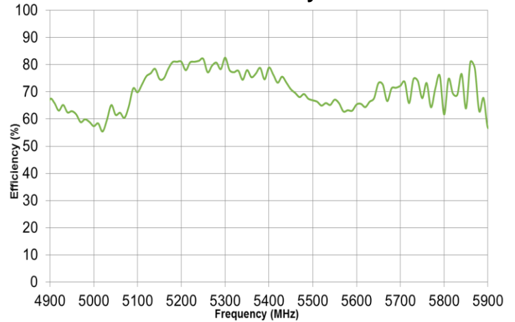
Efficiency
