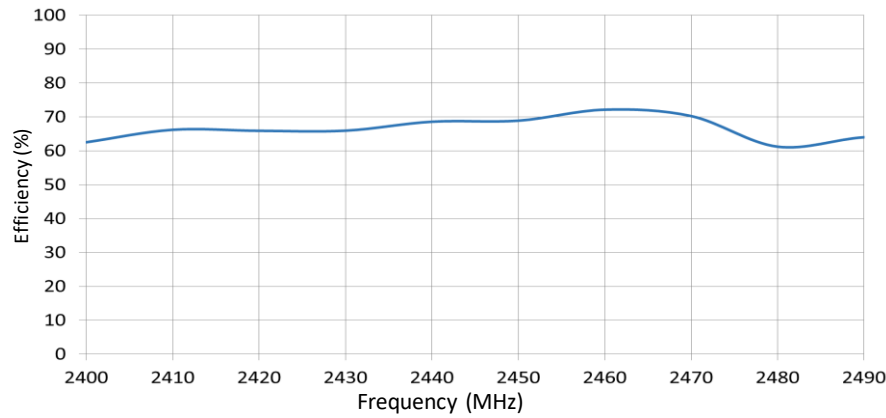
Efficiency (2.400 – 2.490) GHz
