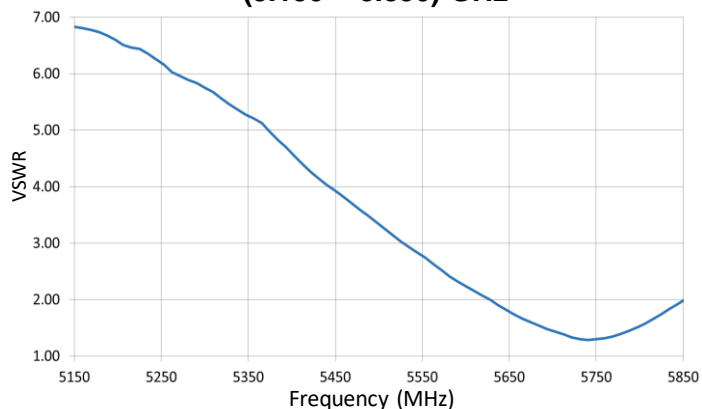
VSWR (5.150 – 5.850) GHz
