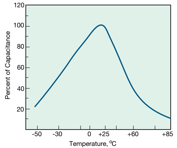
Typical Temperature Characteristic Y5V
