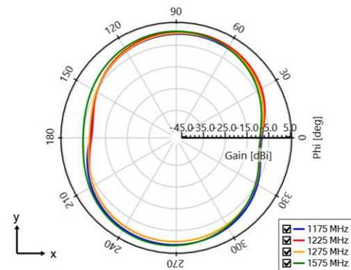
M830120-02_B - Gain - \theta = 90 deg [Plane XY]
