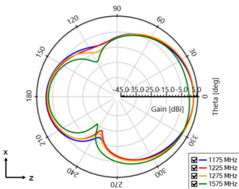
M830120-02_B - Gain - \phi = 0 deg [Plane XZ]
