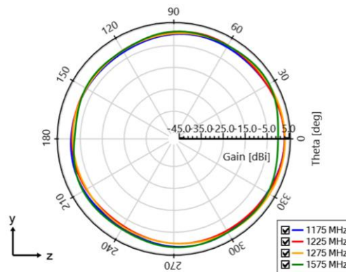
M830120-02_B - Gain - \phi = 90 deg [Plane YZ]
