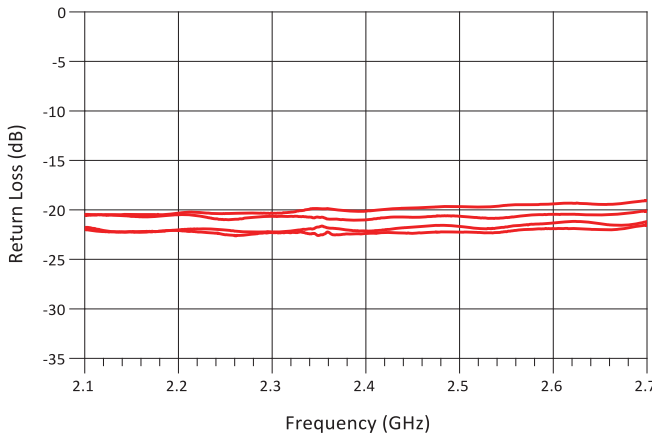
Return Loss
