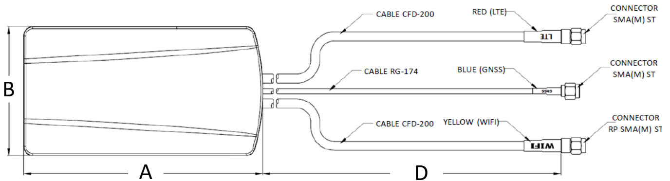
Top View
