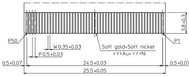
DETAIL C(5:1)
