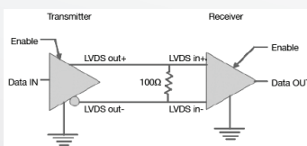
LVDS Interface
