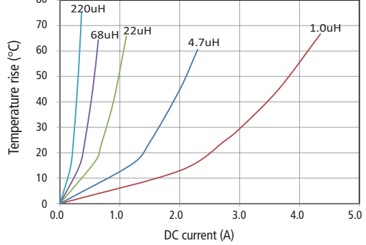
TYS4020 Temperature Rise vs DC Current
