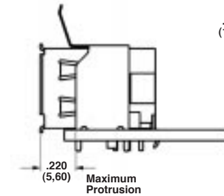
Side View: Connector Gasket Assembly
