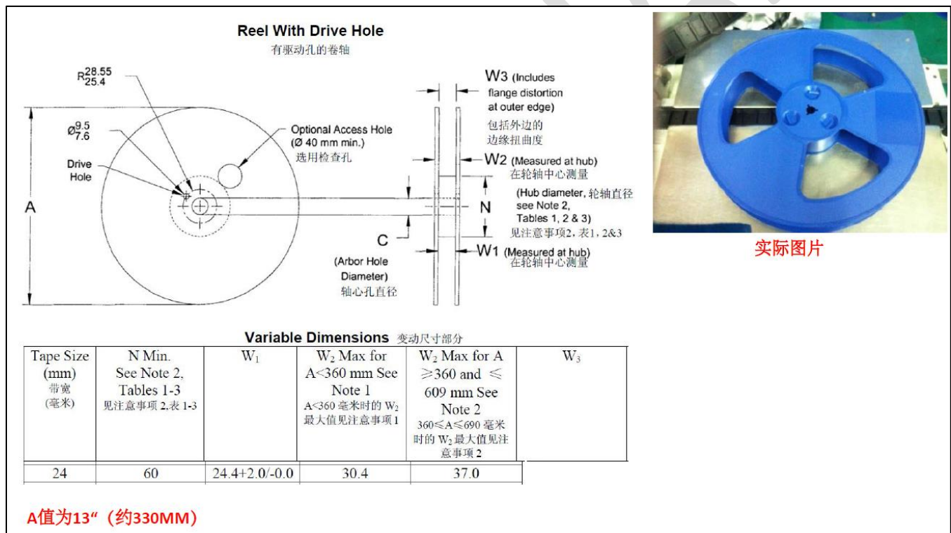
Figure 10: Reel specifications
