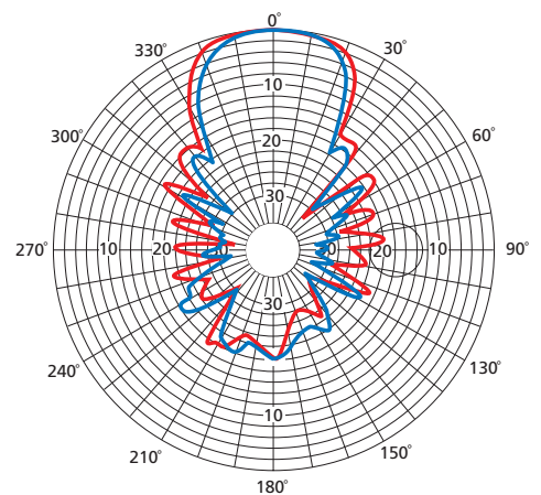
TYPICAL 13 ELEMENT
