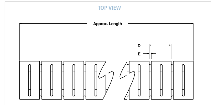
DUAL SLOT SERIES DIMENSIONS
