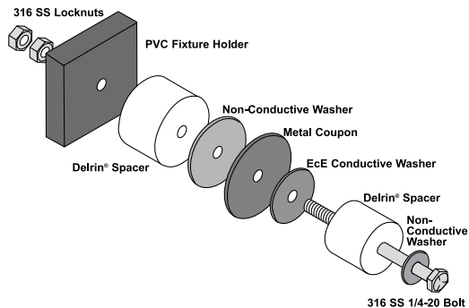
FIGURE 2. CONDUCTIVE WASHER
