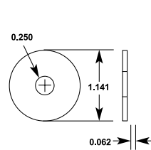
FIGURE 2. CONDUCTIVE WASHER
