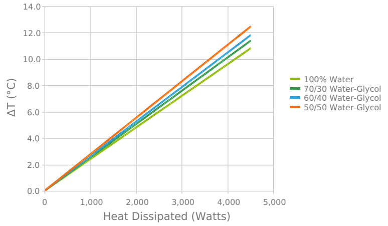
WL3004 Fluid Inlet/Outlet Temperature Difference (ΔT) @ Nominal Flow 6 L/min
