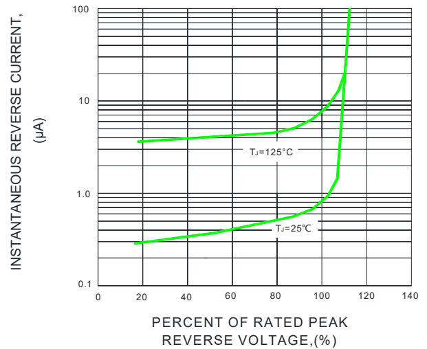
FIG.4-TYPICAL REVERSE CHARACTERISTICS
