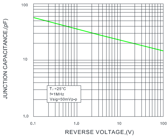
FIG.5-TYPICAL JUNCTION CAPACITANCE
