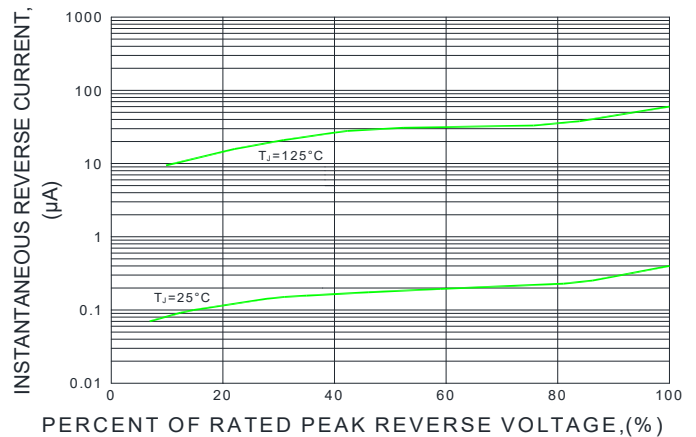
FIG.4-TYPICAL REVERSE CHARACTERISTICS
