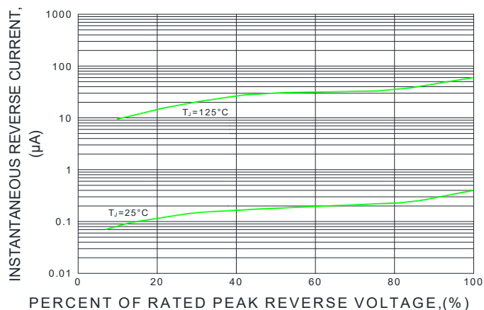
FIG.4-TYPICAL REVERSE CHARACTERISTICS
