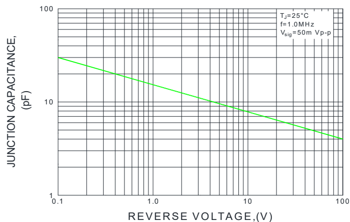
FIG.5-TYPICAL JUNCTION CAPACITANCE
