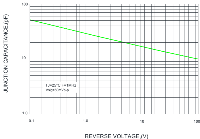
FIG.5-TYPICAL JUNCTION CAPACITANCE
