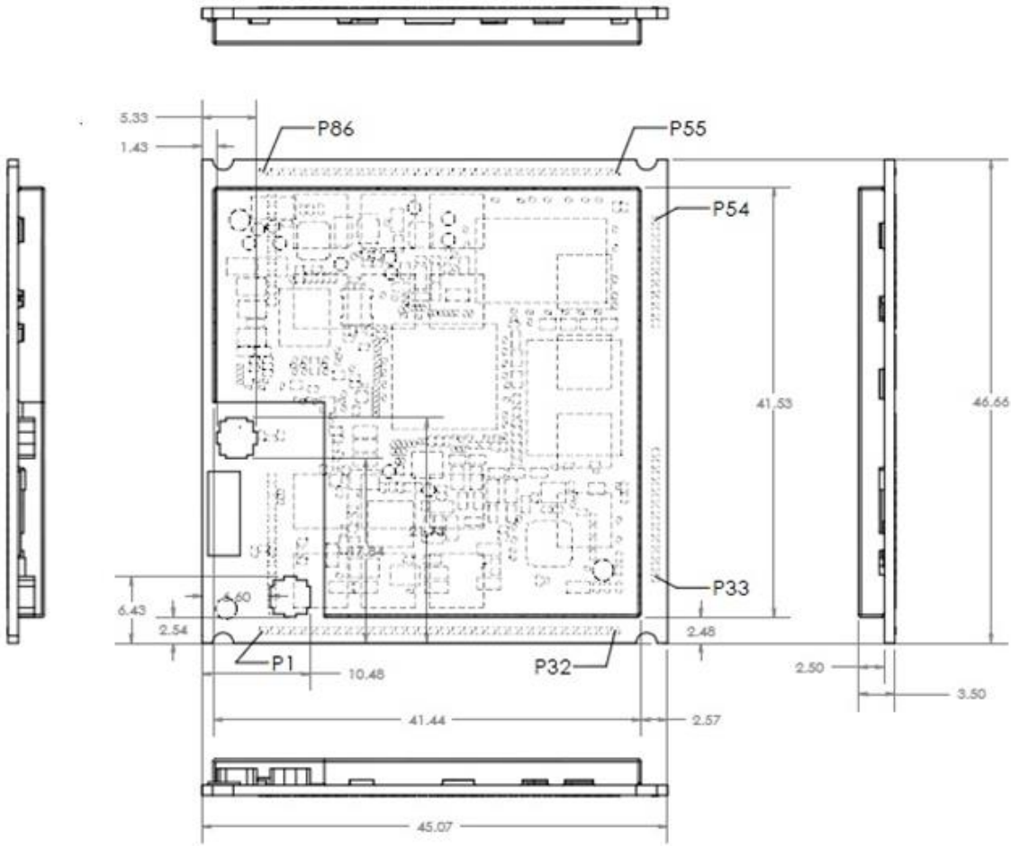
Figure 10 PW20502 Enterprise Wi-Fi IoT Wi-Fi Module
