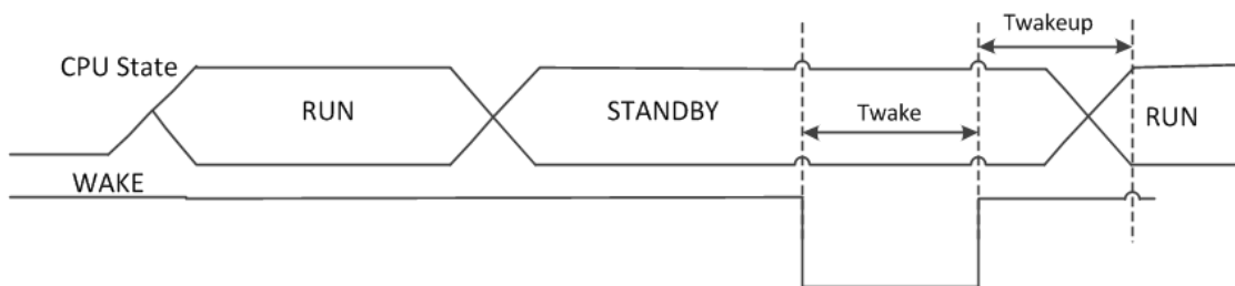
Figure 8 Wake Timing
