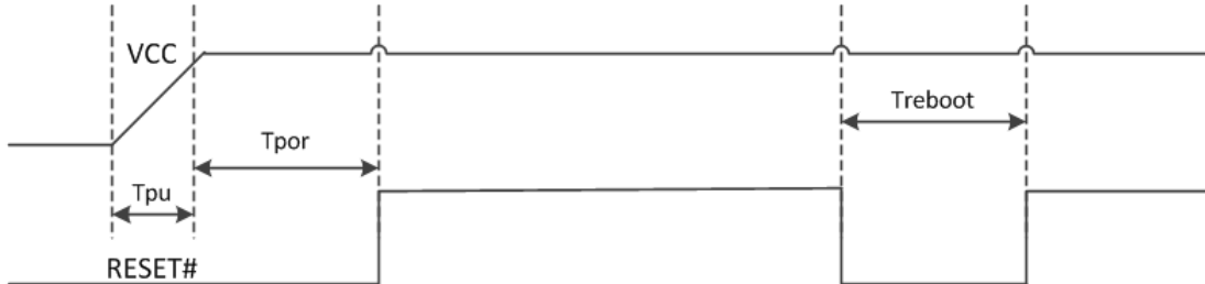
Figure 6 Reset Timing
